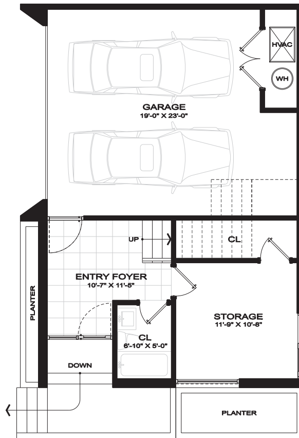
Ground Floor Plan 826sf
